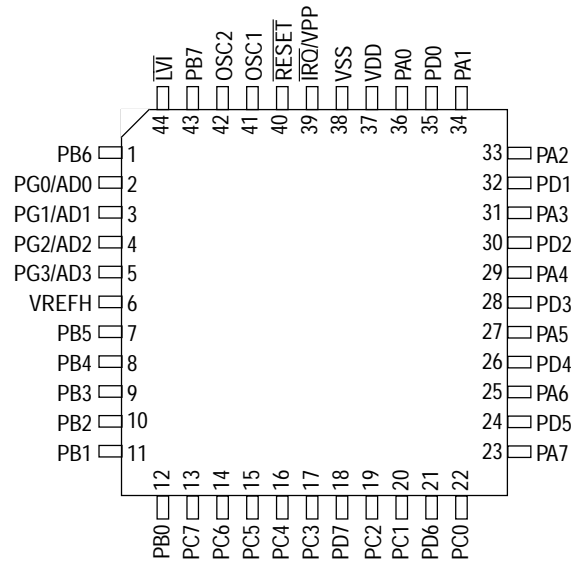
Figure 32 44-pin QFP pinout
