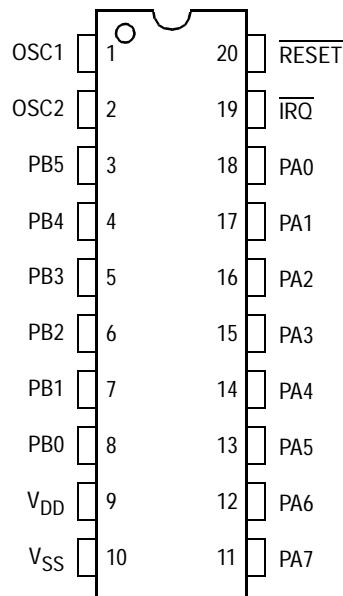
Figure 1-2. Pin Assignments
