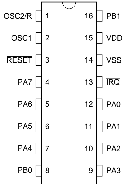
Figure 1-2. Pin Assignment for 16-Pin Package
