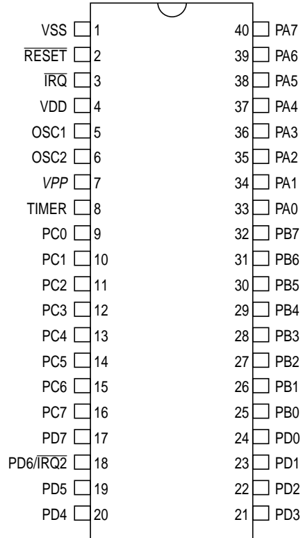
Figure 2-4 Pin Assignment for 40-pin PDIP
