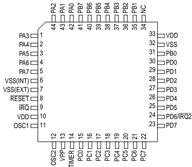
Figure 2-6 Pin Assignment for 44-pin QFP
