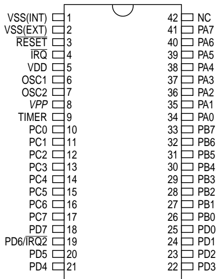
Figure 2-5 Pin Assignment for 42-pin SDIP
