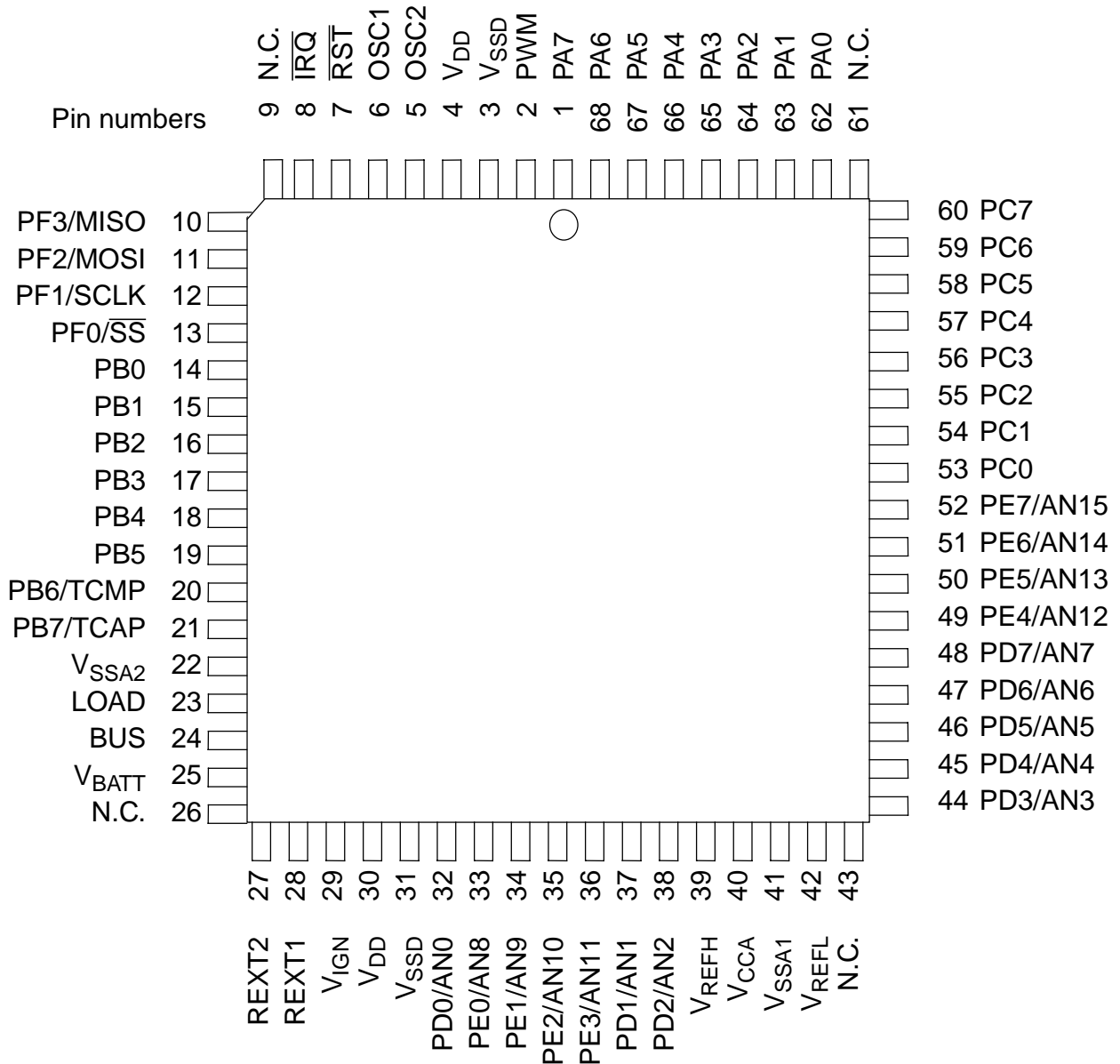
Figure 1-2: MC68HC05V7 Pin Assignments (68-pin PLCC package)
