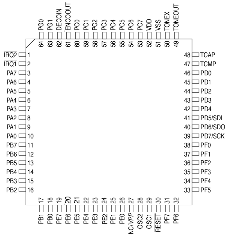
Figure 2-2 Pin Assignments for 64-pin QFP package
