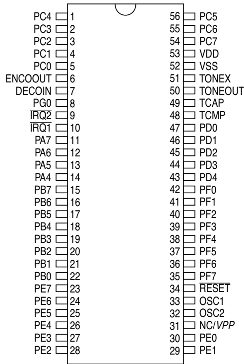
Figure 2-1 Pin Assignments for 56-pin SDIP package
