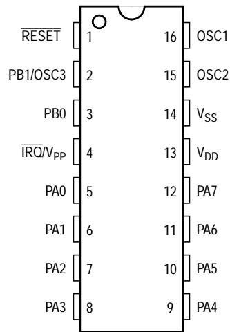
Figure 1-2. Pin Assignments
