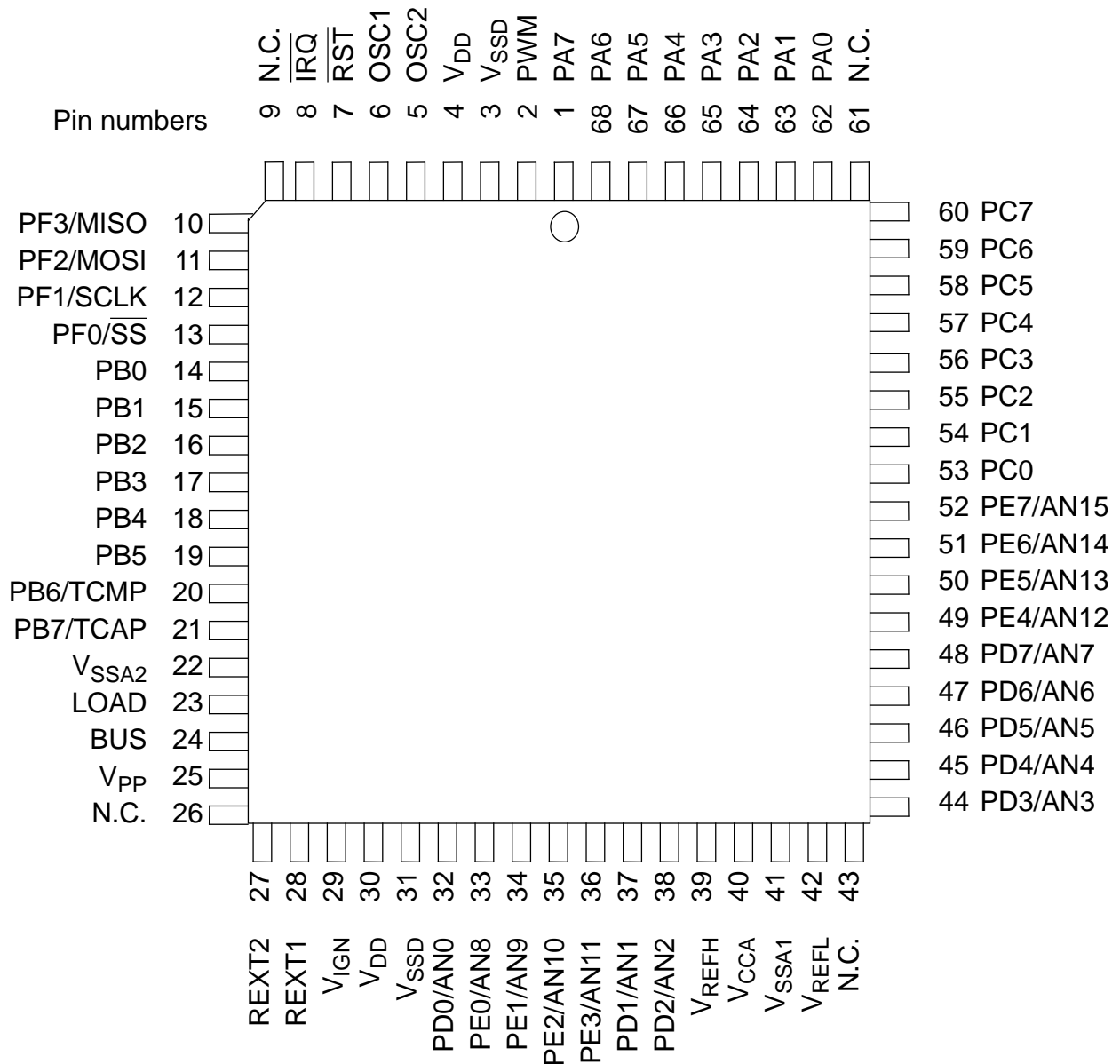
Figure 1-2: MC68HC705V8 Pin Assignments (68-pin PLCC package)
